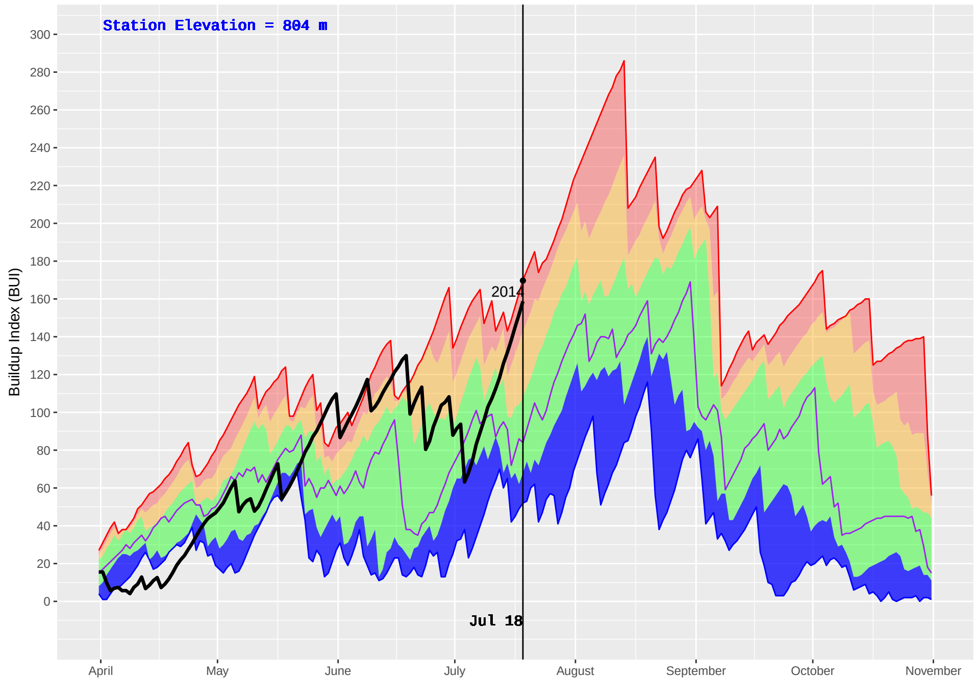
KOOCANUSA (1075) : Historical (2010–2016) and Current (2018) Daily Buildup Index (BUI)
